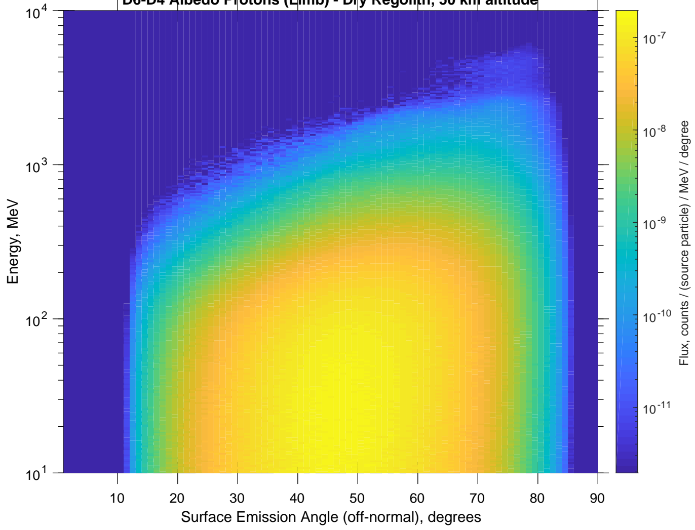
D6-D4 Albedo Protons (Limb) - Dry Regolith, 50 km altitude
