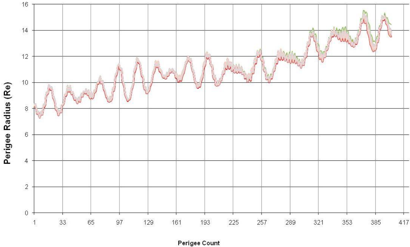
IBEX Full Monte Carlo Perigee History (425 Runs, 255 Shown)
