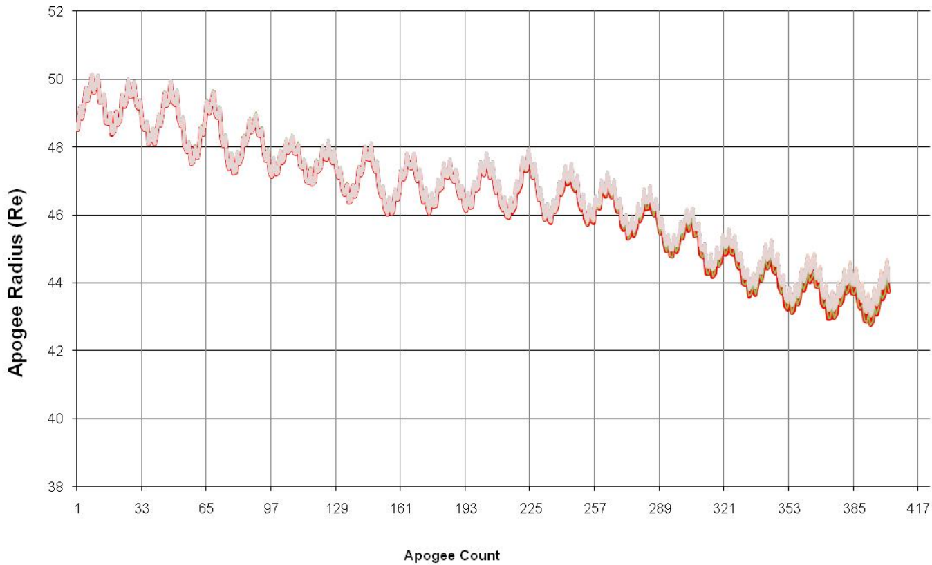
IBEX Full Monte Carlo Apogee History (425 Runs, 255 Shown)
