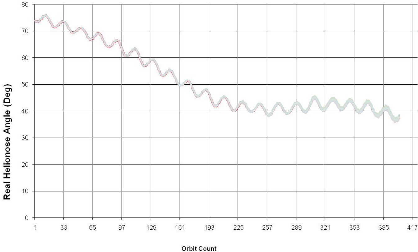
IBEX Full Monte Carlo Real Helionose Angle History (425 Runs, 255 Shown)
