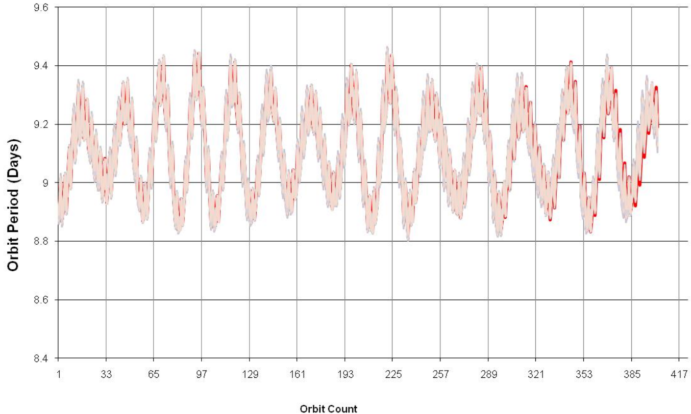
IBEX Full Monte Carlo Orbit Period History (425 Runs, 255 Shown)
